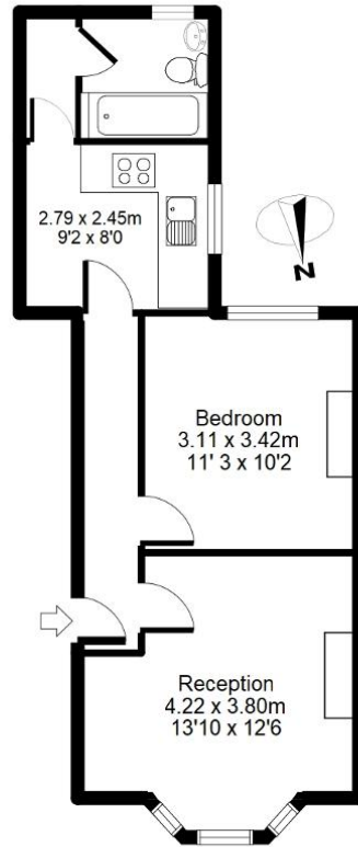
APPROX GROSS INTERNAL FLOOR AREA: 437 sq. ft / 41 sq. m
